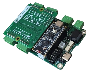
IoTbase Nano with the IoTextra Input module
